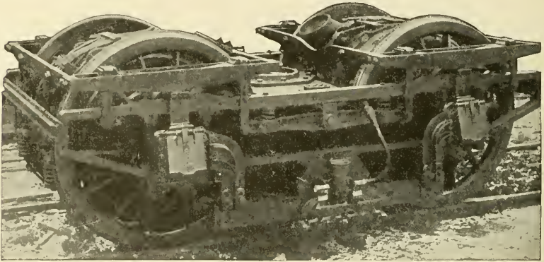
Fig. 257. View of Truck Showing Spring Supports for Motor
